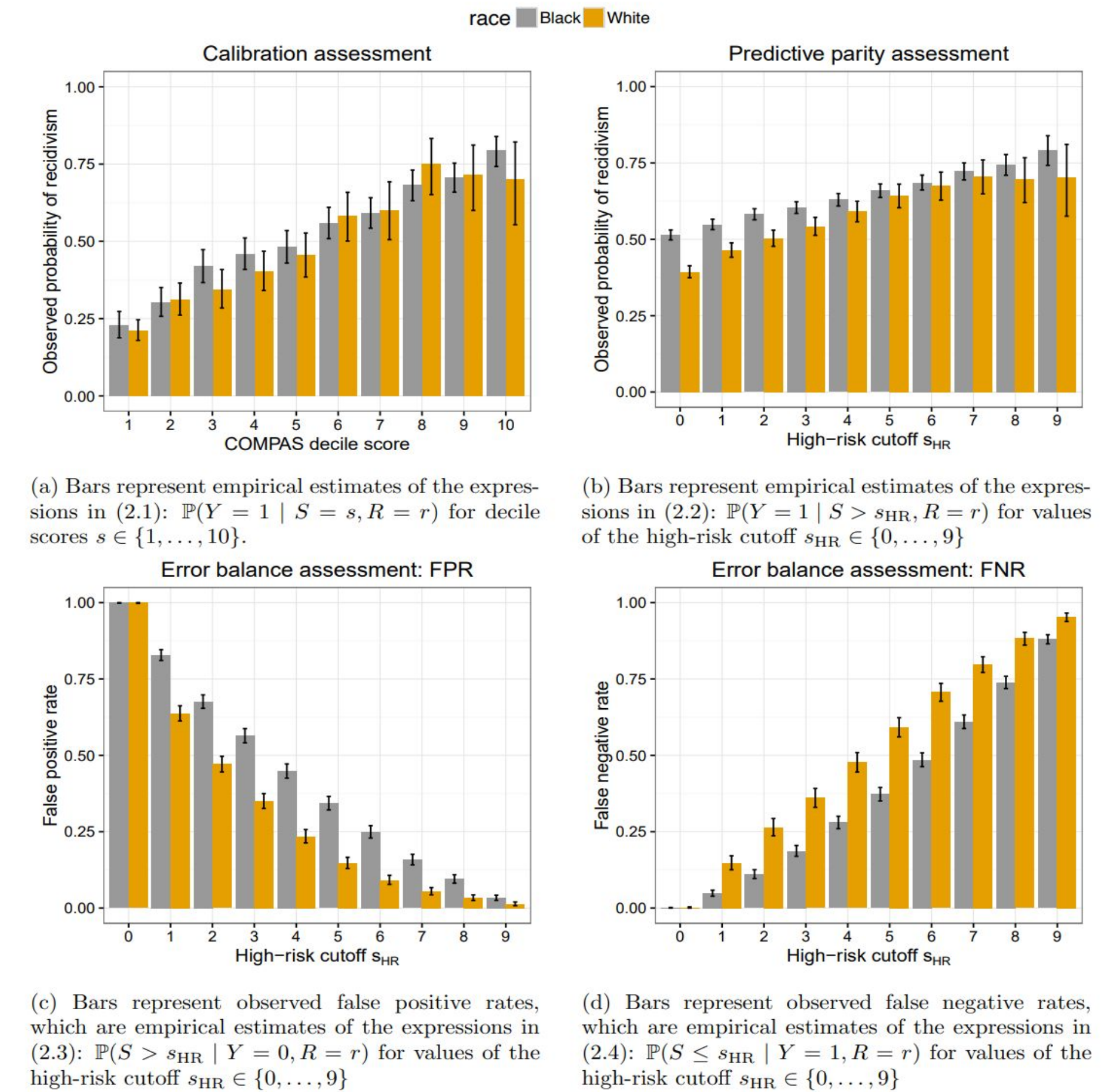
Figure III. Empirical assessment of the COMPAS RPI according to three of the fairness criteria presented in Section 2.1. Error bars represent 95% confidence intervals. These Figures confirm that COMPAS is (approximately) well-calibrated, satisfies predictive parity for high-risk cutoff values of 4 or higher, but fails to have error rate balance (Fair prediction with disparate impact: A study of bias in recidivism prediction instruments by Alexandra Chouldechova).
