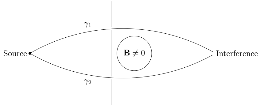
FIGURE 6. The Aharonov-Bohm effect
